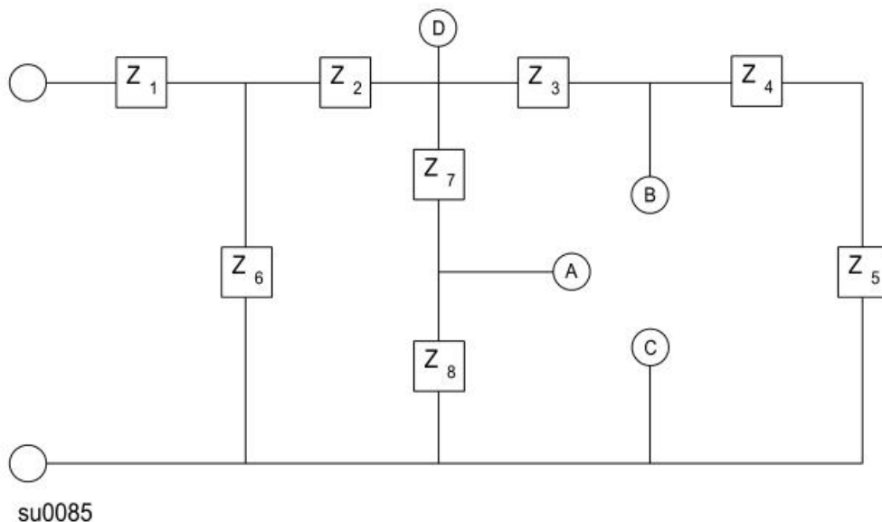
Figure SB9.1 Example of an electronic circuit with low-power points
