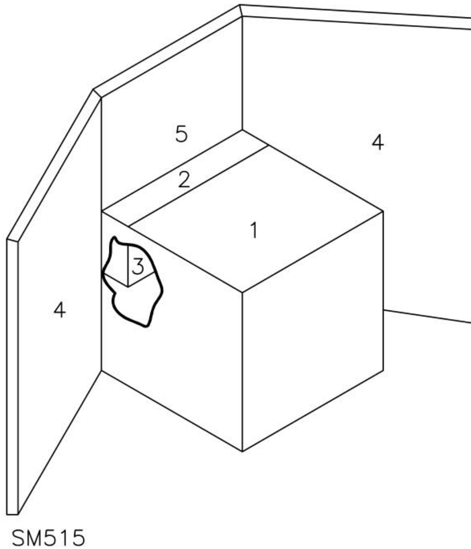
Figure 186.1 Test enclosure for down-draft fan
