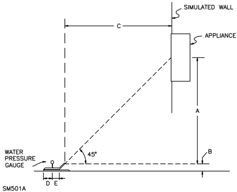
Figure 181.2 Water spray test set-up for wall-insert fans
