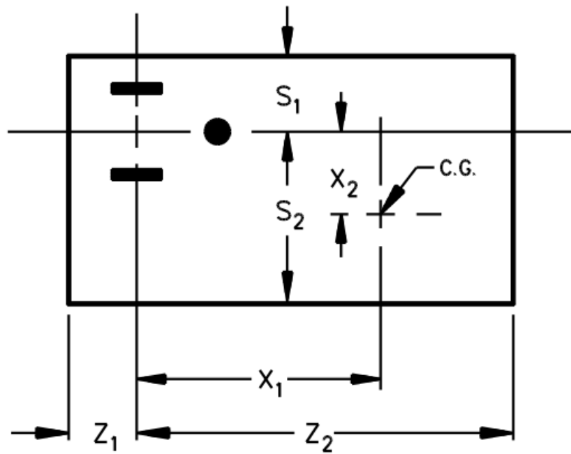
Figure 209.1 Dimensions of a plug-in product
