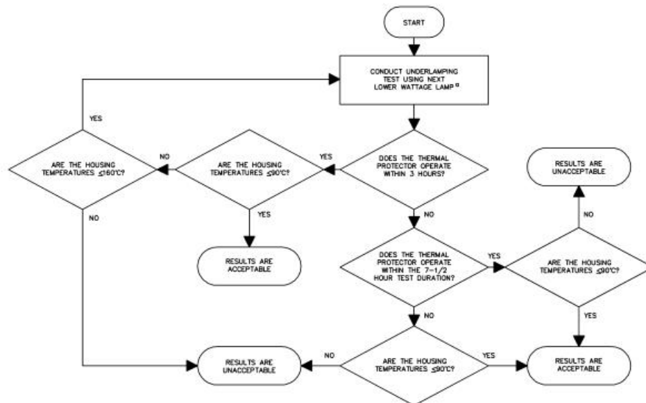
Figure 144.1 Flow chart for underlamping test procedure
