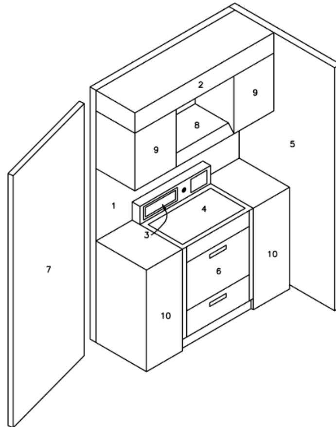
Figure 129.1 Test enclosure for ventilating-hood-fan shelf over counter level range
