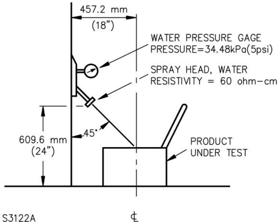
Figure 157.1 Set-up for water spray test
