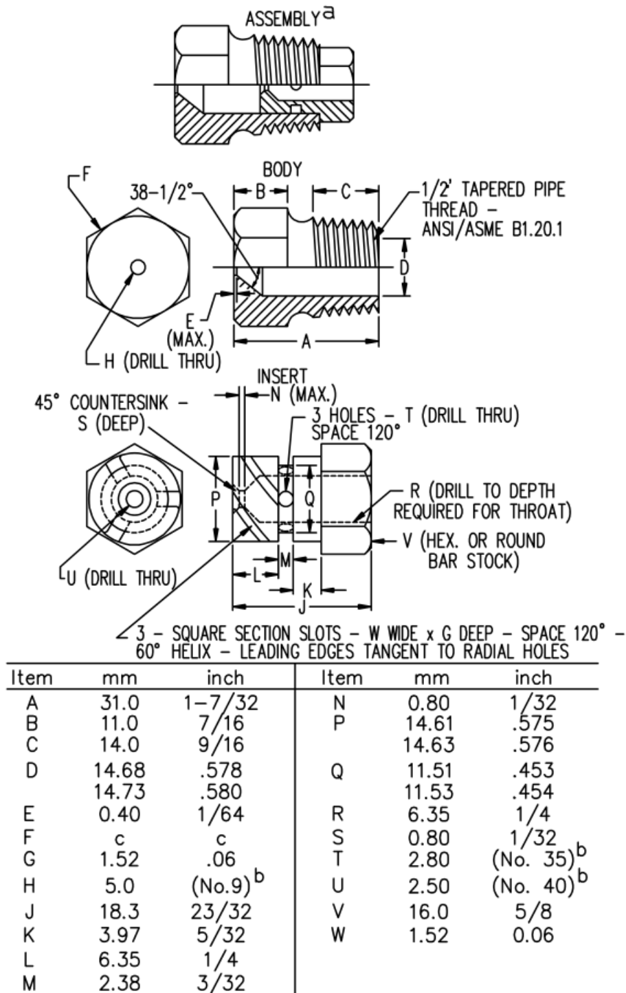
Figure 48.2 Spray head assembly
